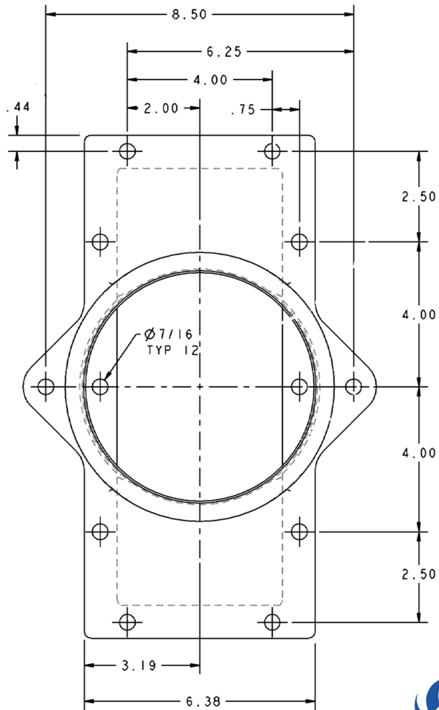
CONNECTOR, INLET/DISCHARGE 412 ROOTS-FLO
