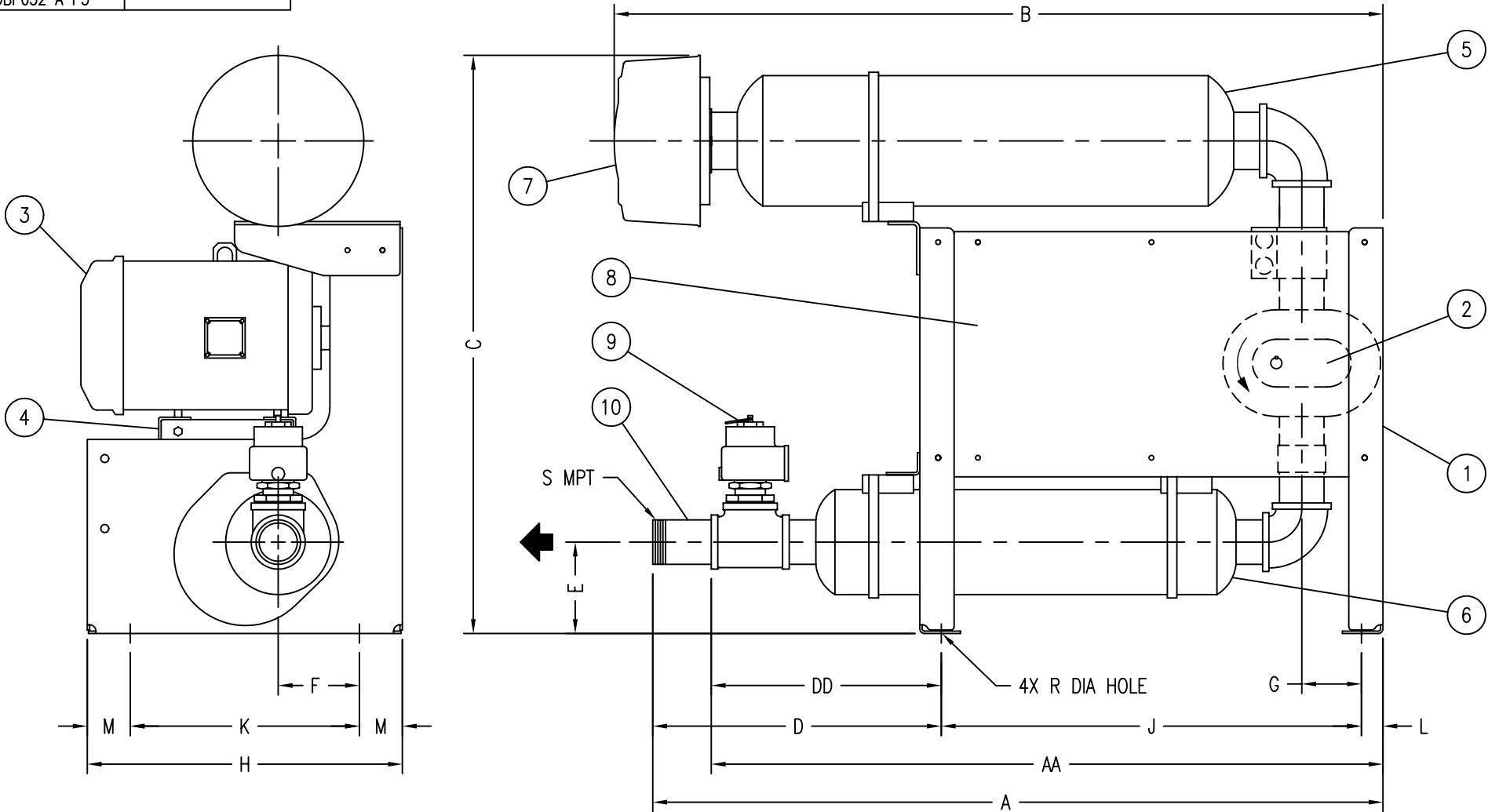
FIGURE 2, CCF FILTER, LARGER/EQUAL
