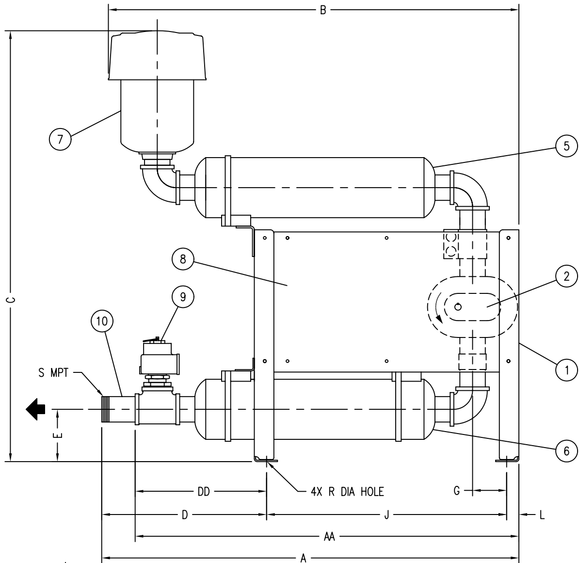
FIGURE 17, CCS FILTER/SILENCER, EQUAL/EQUAL
