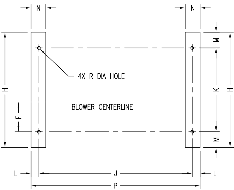
BASE ANCHOR BOLT & FOOTPRINT PATTERN DIMENSION TOLERANCE: \pm 1/4
