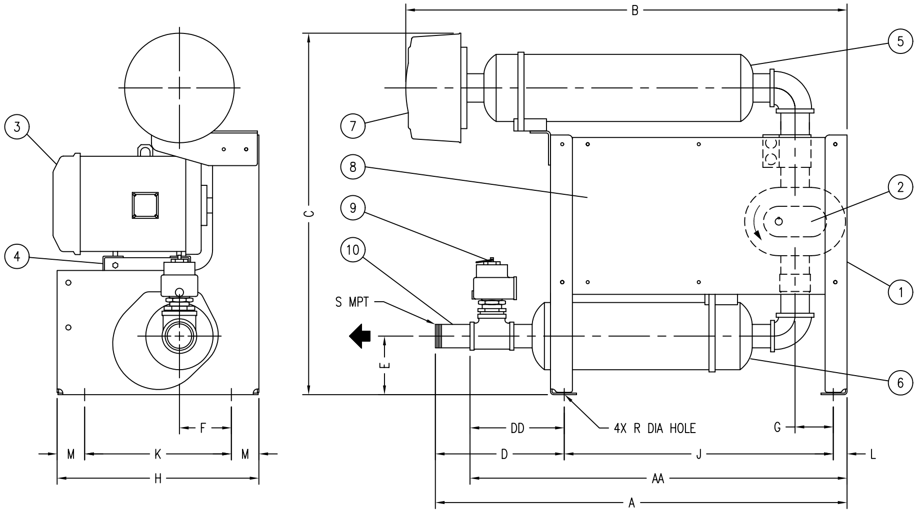
FIGURE 3, CCF FILTER, EQUAL/SMALLER
