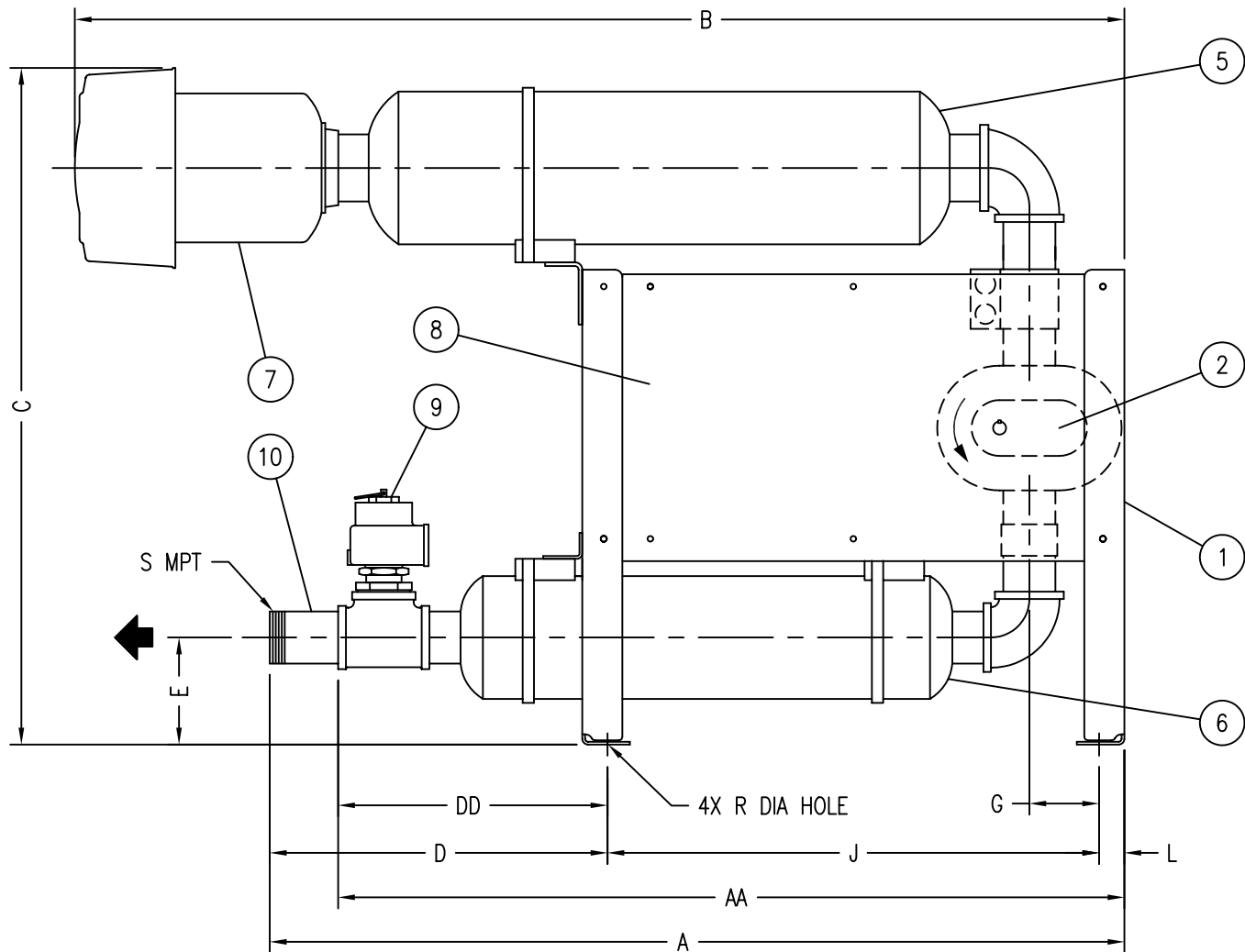
FIGURE 5, CCS FILTER/SILENCER, LARGER/EQUAL
