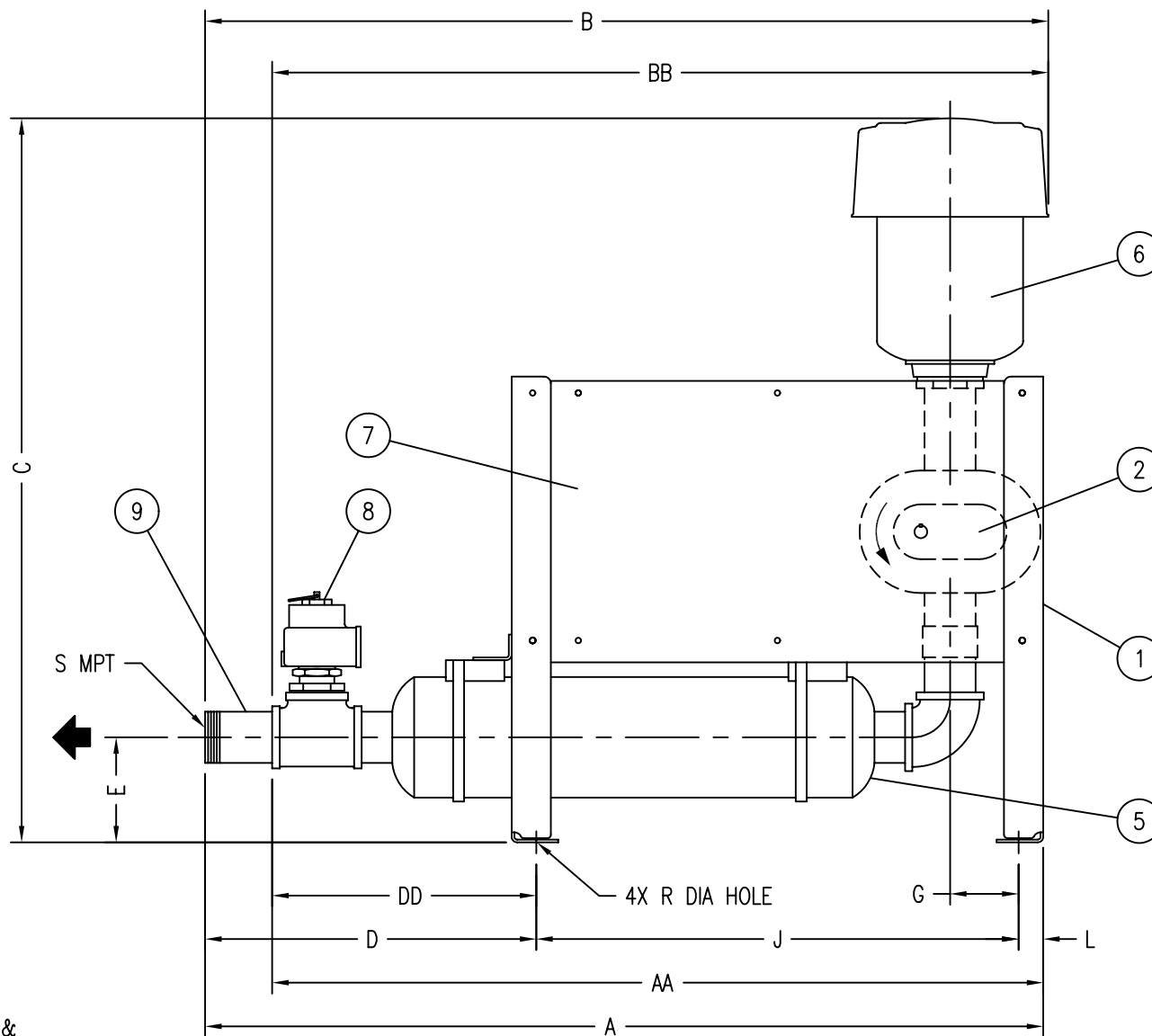
FIGURE 8, CCS FILTER/SILENCER, LARGER/EQUAL
