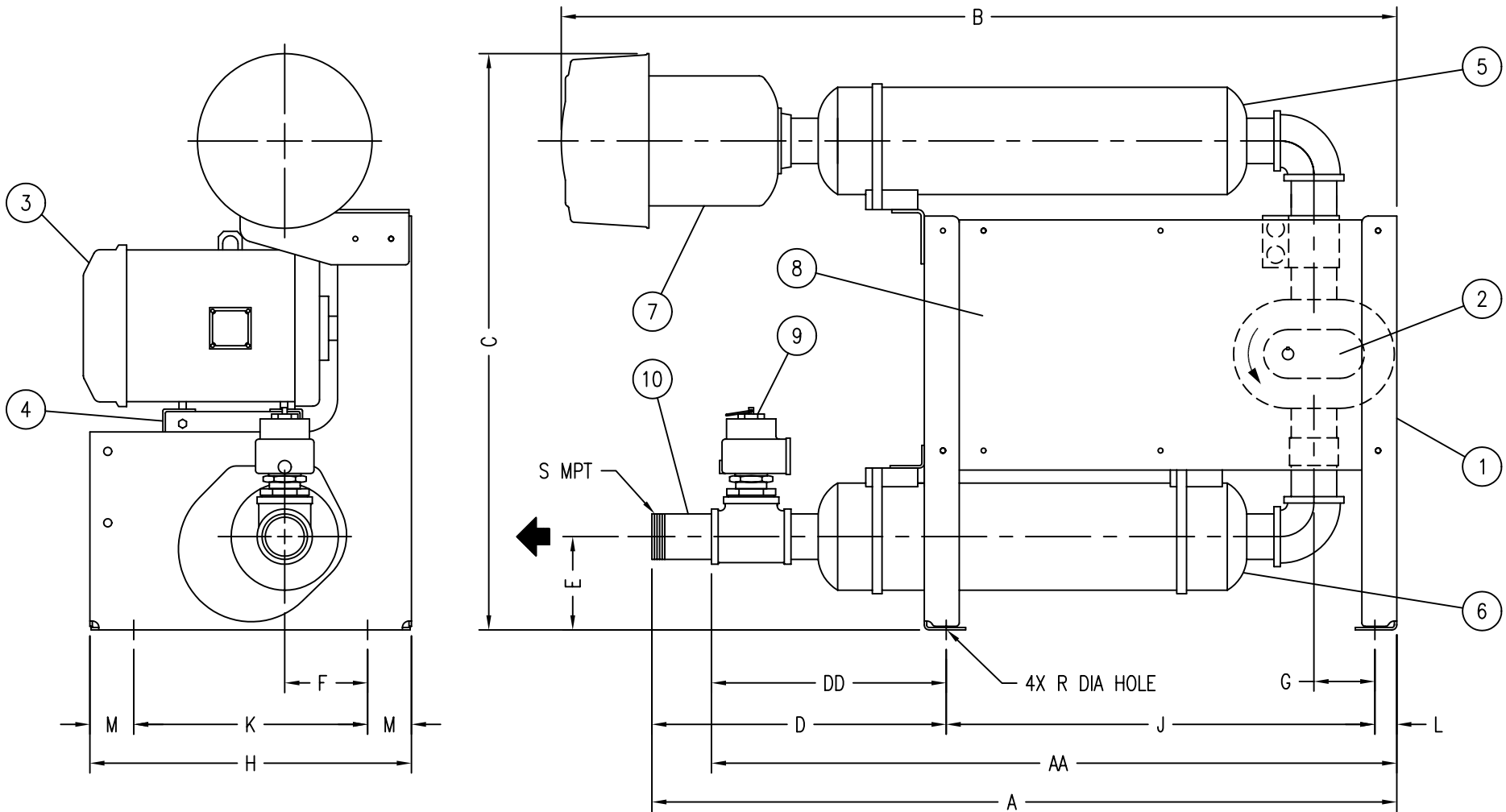
FIGURE 4, CCS FILTER/SILENCER, EQUAL/EQUAL
