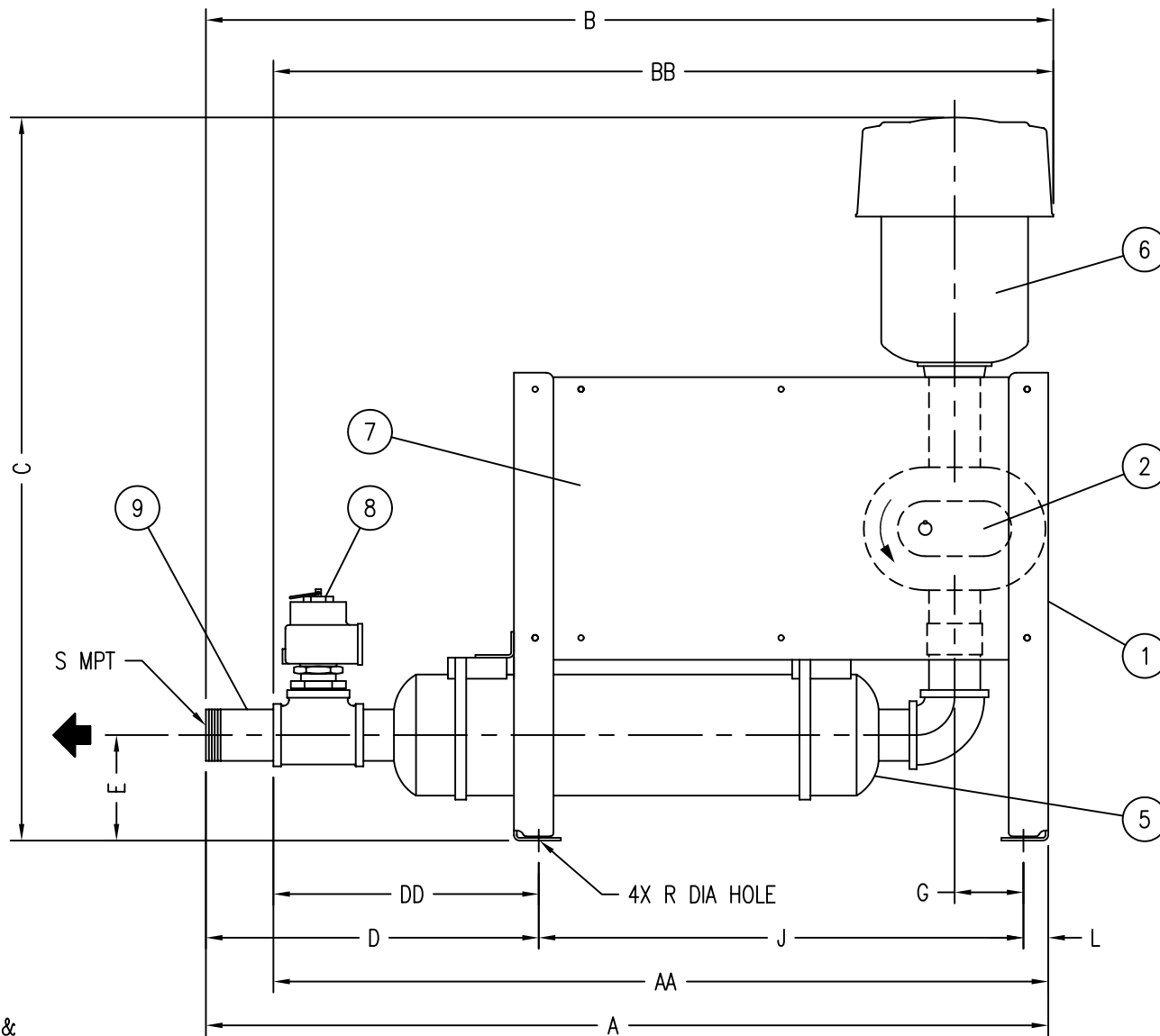
FIGURE 7, CCS FILTER/SILENCER, EQUAL/EQUAL
