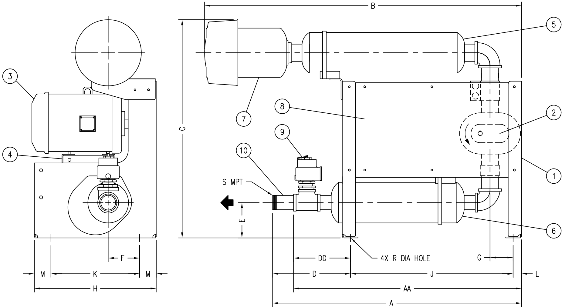
FIGURE 6, CCS FILTER/SILENCER, EQUAL/SMALLER
