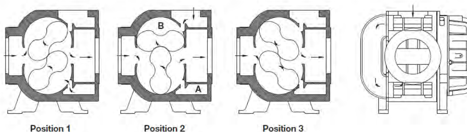
Figure 1 - Flow Through an RVS/VJ Blower
