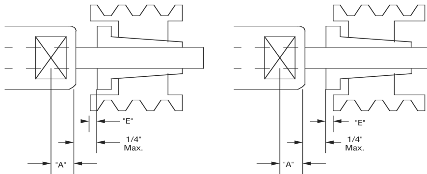
Sheave Type 1
