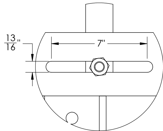
DETAIL A BOLT SLOTS (4x TYP) SCALE 1 : 4
