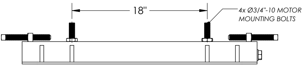
FRONT VIEW
