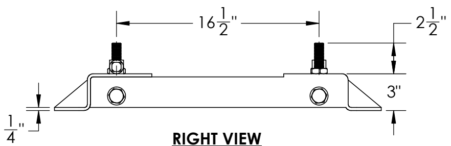
RIGHT VIEW
