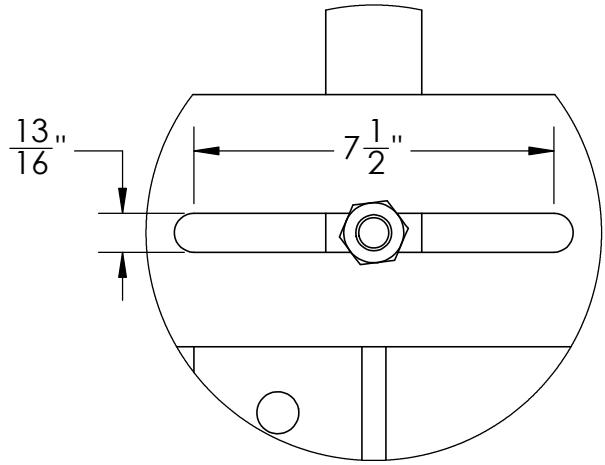
DETAIL A BOLT SLOTS (4x TYP) SCALE 1 : 4
