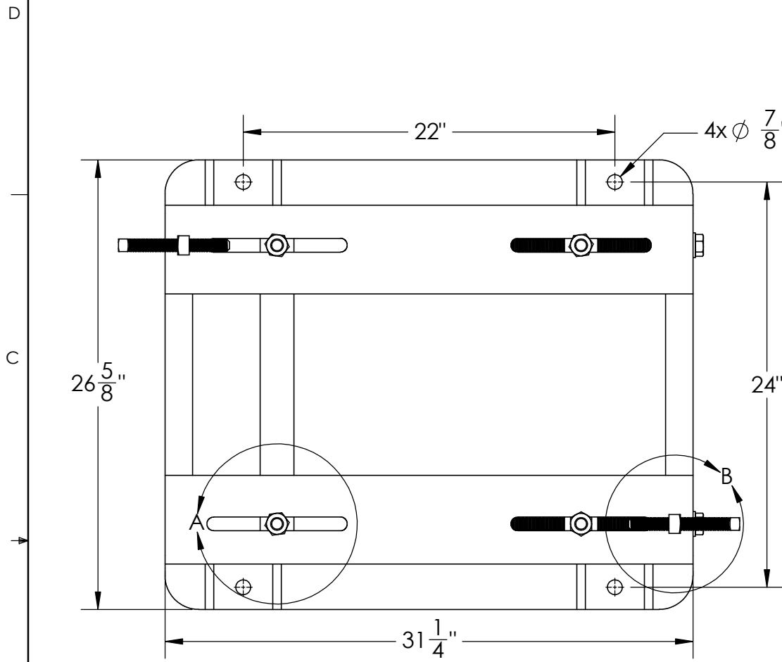
TOP VIEW
