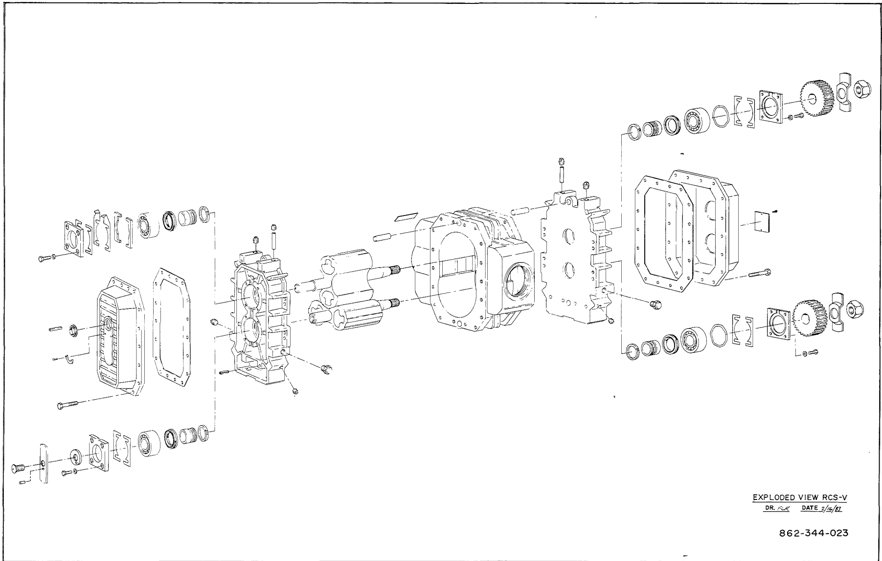
Figure 10 — Exploded View
