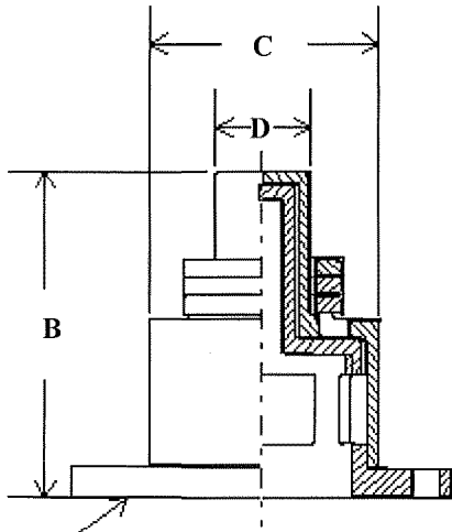
A, Mounting Flange, ASA 125# Drilling USE ONLY FULL FACE GASKET
