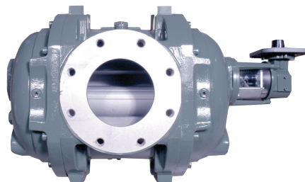
Series B3 23M/38M/56M Meter
