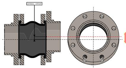
Figure 5: Lateral Misalignment
