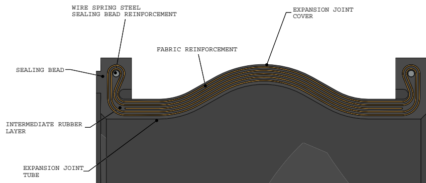
Figure 8: Rubber Expansion Joint General Materials of Construction
