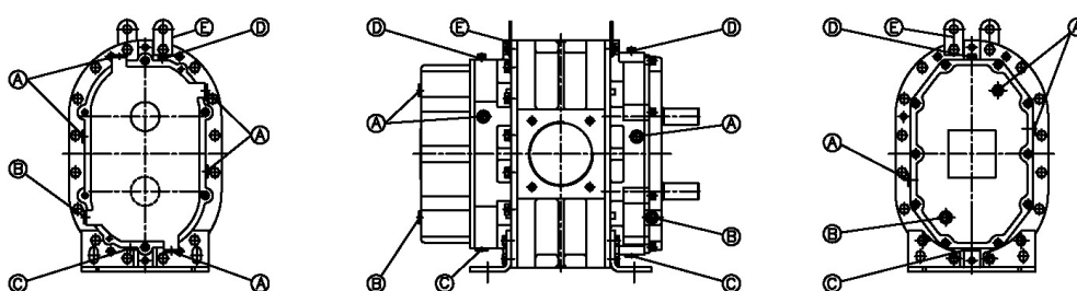
A: PLUG B: OIL LEVEL GAUGE C: PLUG MAGNETIC D: BREATHER(Oil fill plug top) E: LIFTING LUG
