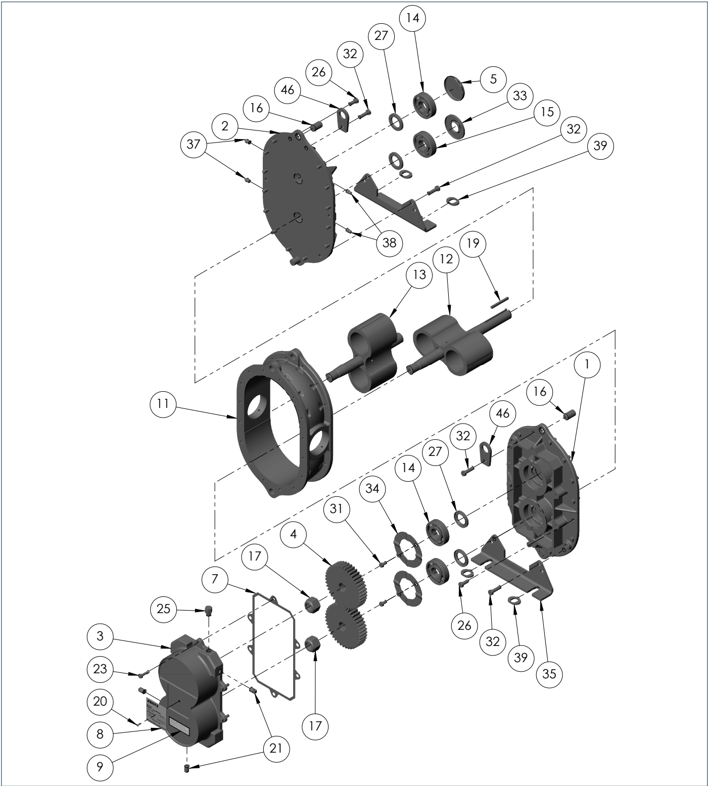
Assembly of Roots Universal RAI Series, Air Blowers, 2-1/2" through 5" gear diameter
