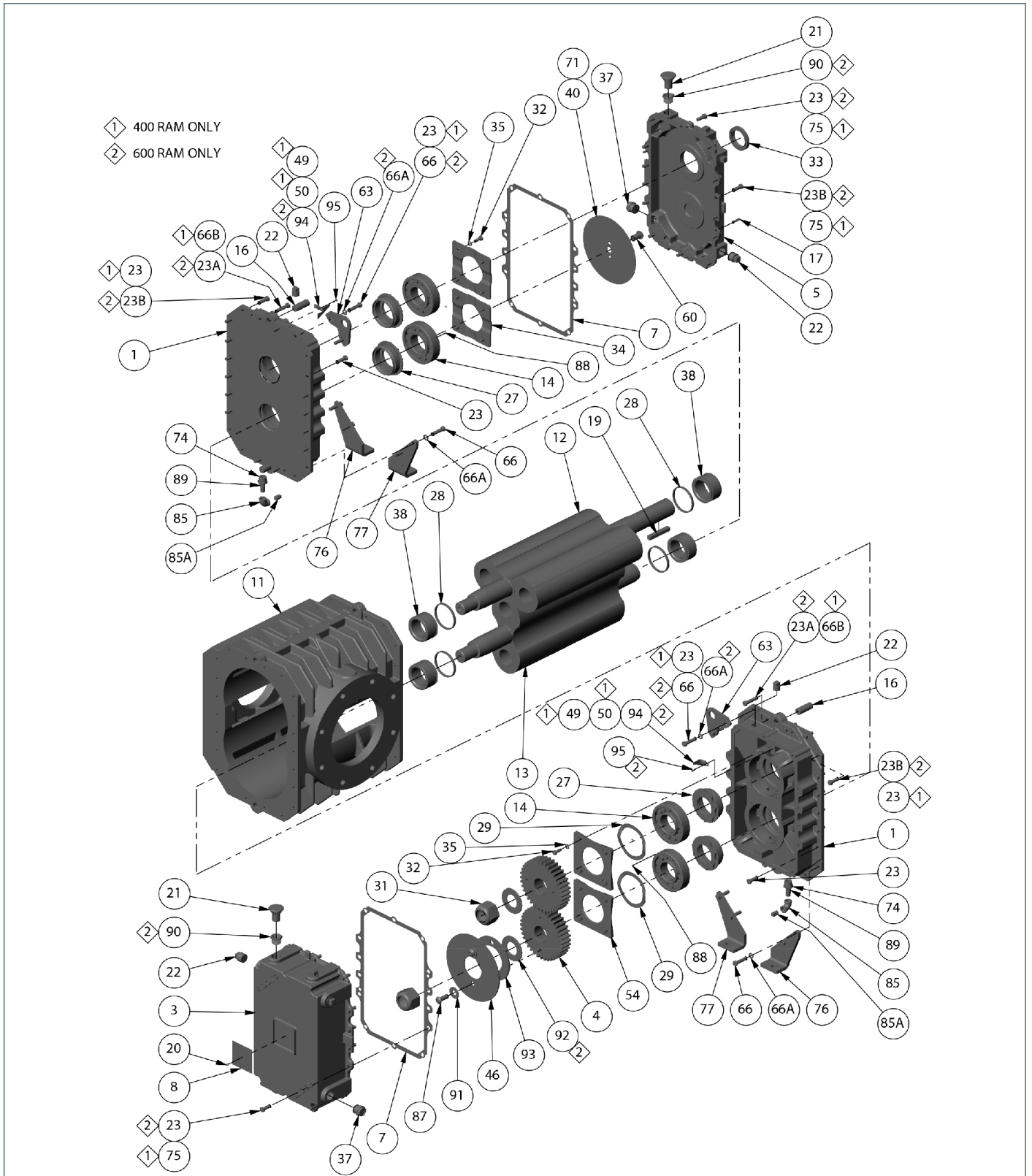
Assembly of Roots 400 & 600 RAM-G & RAM-GJ
