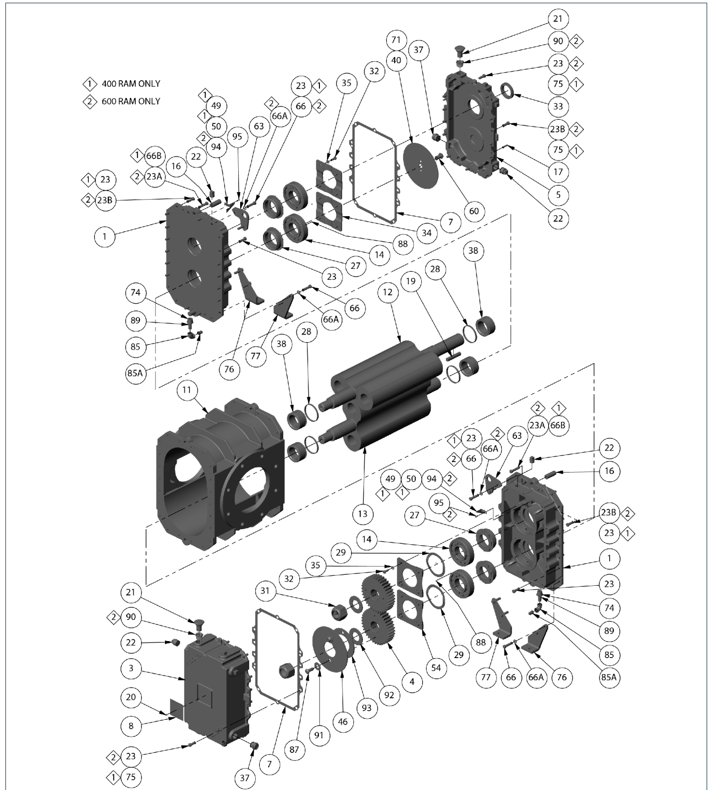
Assembly of Roots 400 & 600 RAM & RAM-J
