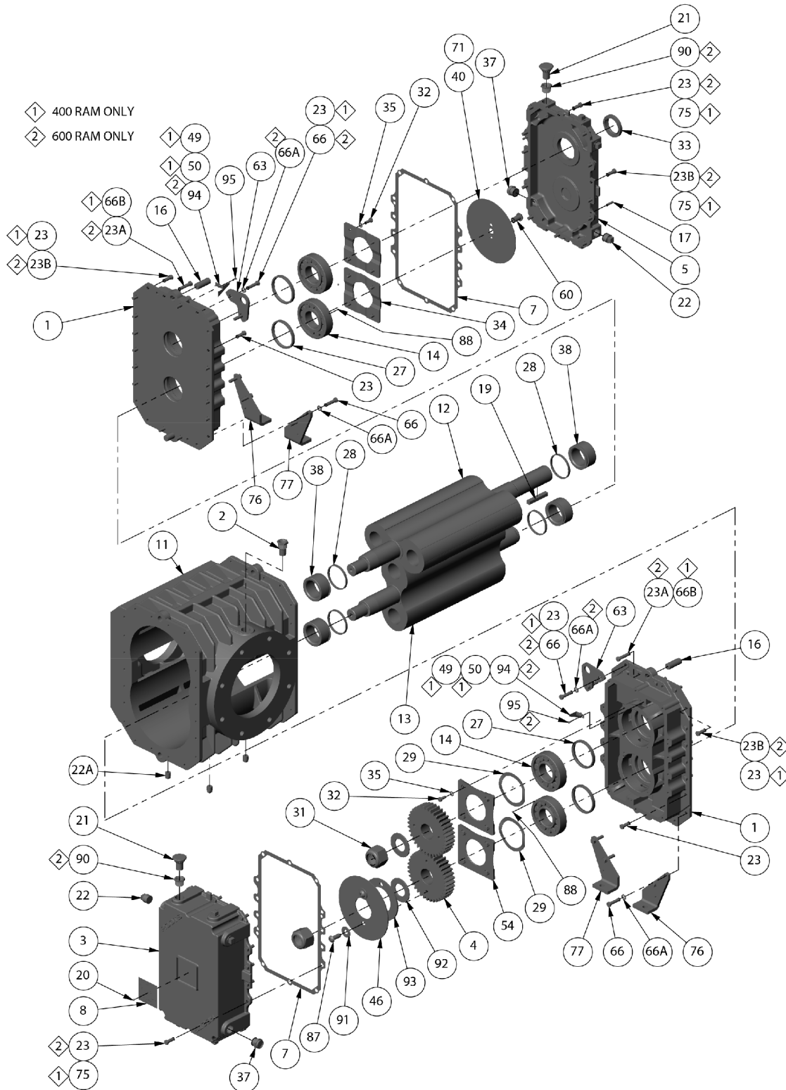
Assembly of Roots 400 & 600 RAM-VJ
