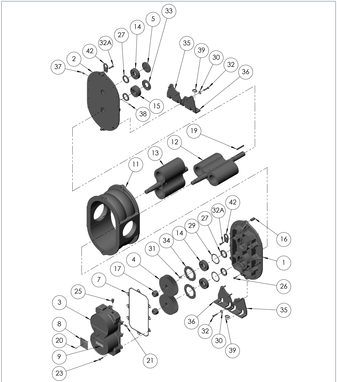
Assembly of Roots Universal RAI Series, Air Blowers, 6" through 7" gear diameter
