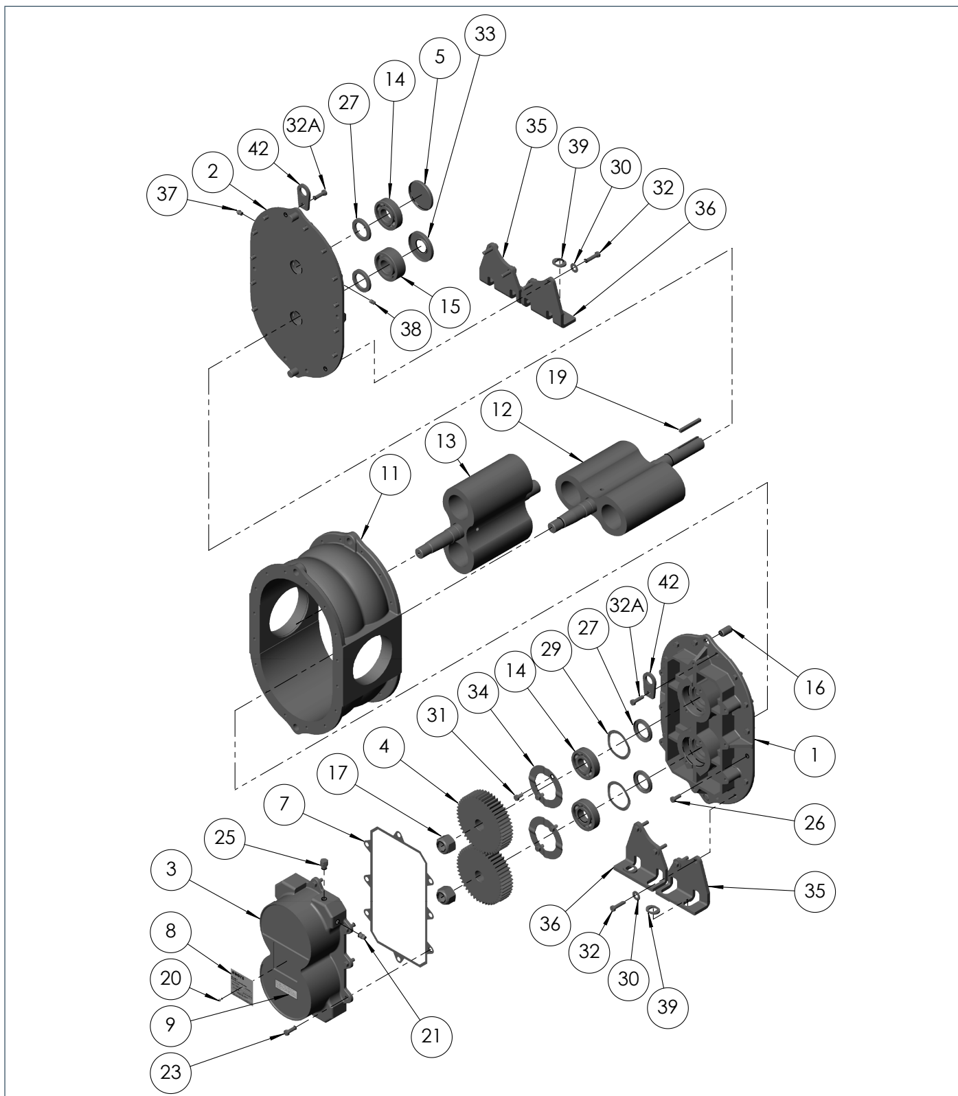
Assembly of Roots Universal RAI Series, Air Blowers, 6" through 7" gear diameter
